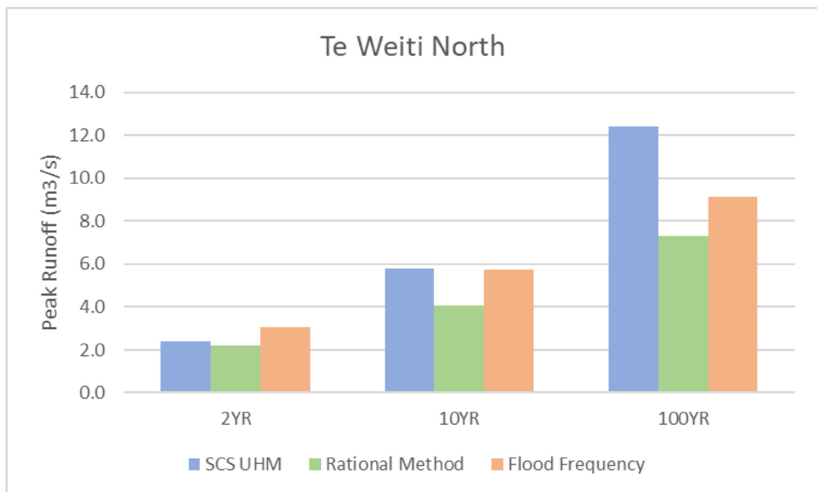
Figure 4-1 Te Weiti North Peak Flow Validation
