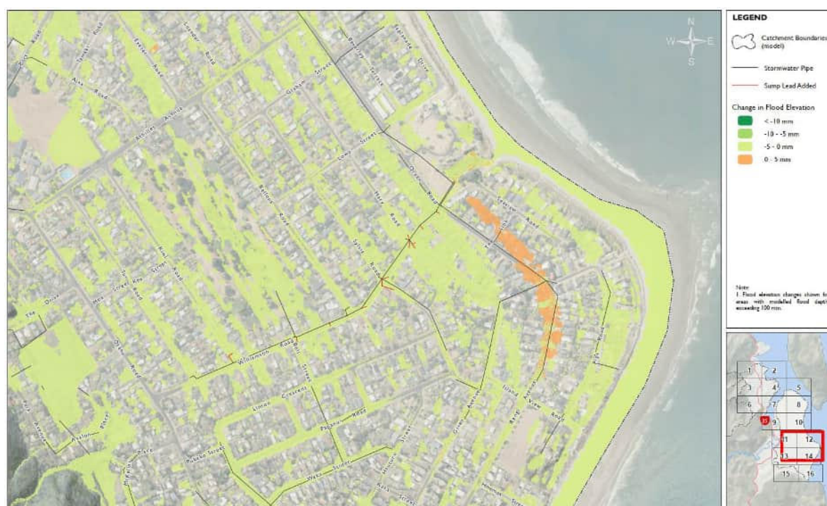
Figure 4-4 Sensitivity Run - Modelling Catchpits near Williamson Park
