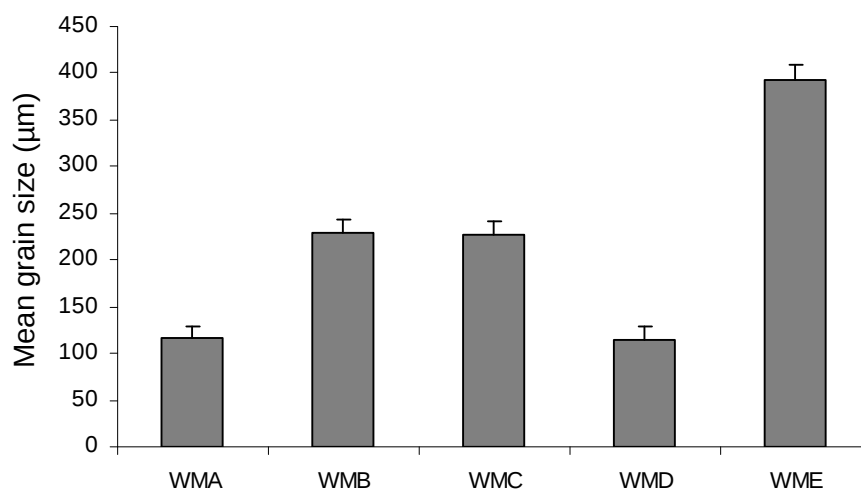
Figure 3: Mean grain size (bars indicate standard error) at sites WMA (cleared and mown 2005); WMB (cleared 2005); WMC (cleared 2007), WMD (intact mangrove) and WME (unvegetated intertidal flat).
