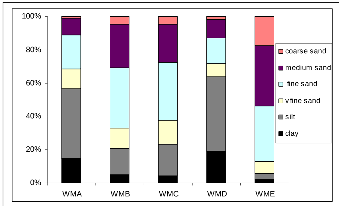
Figure 4: Surface sediment composition (% clay, silt, fine, medium and coarse sand) at sites WMA (cleared and mown 2005); WMB (cleared 2005); WMC (cleared 2007), WMD (intact mangrove) and WME (unvegetated intertidal flat).
