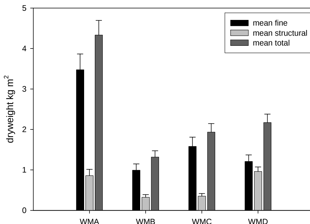
Figure 5: Dry weight ( \text{kg m}^{-2} ) of below-ground biomass, structural roots and fine roots at sites WMA (cleared and mown 2005); WMB (cleared 2005); WMC (cleared 2007) and WMD (intact mangrove habitat).
