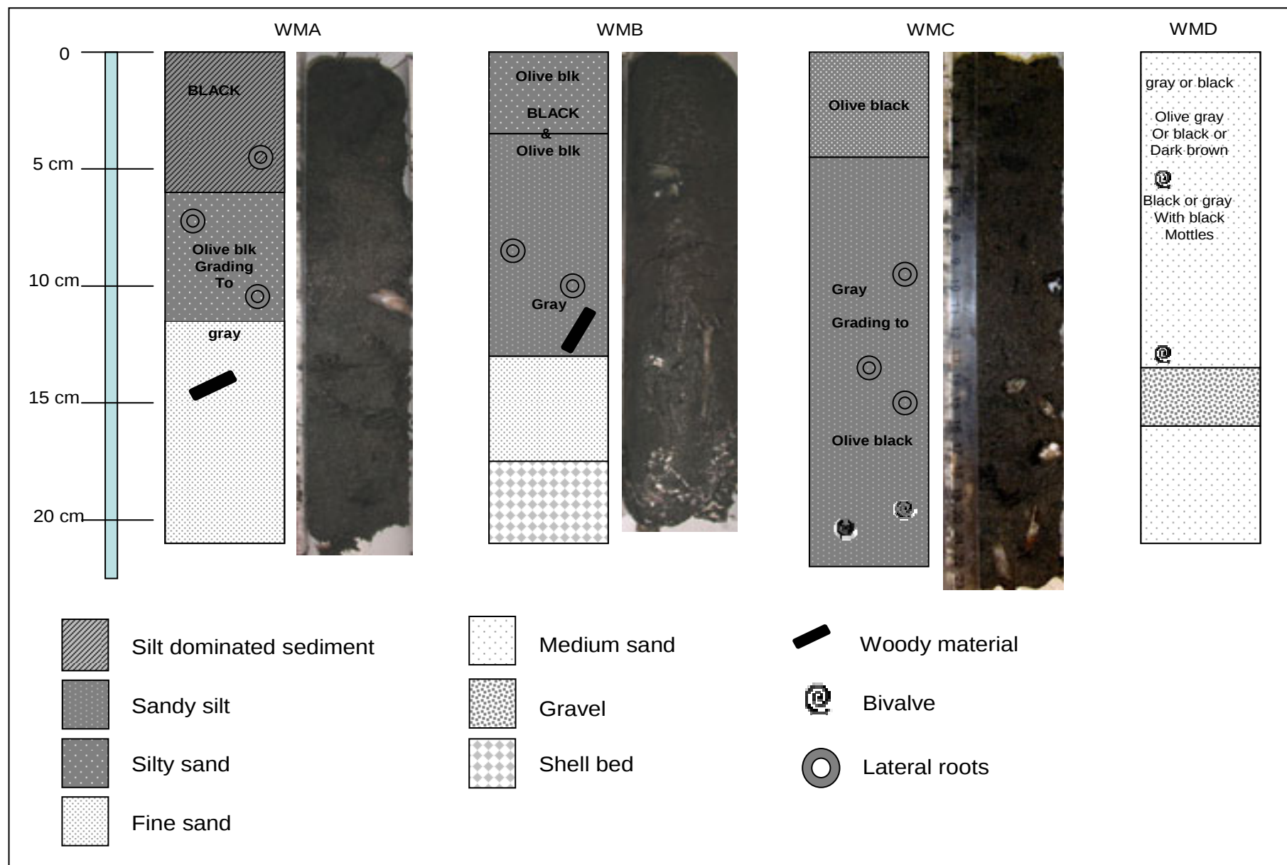
Figure 2: Representative core stratigraphy of each cleared site (WMA, WMB and WMC) and the unvegetated intertidal habitat (WME)
