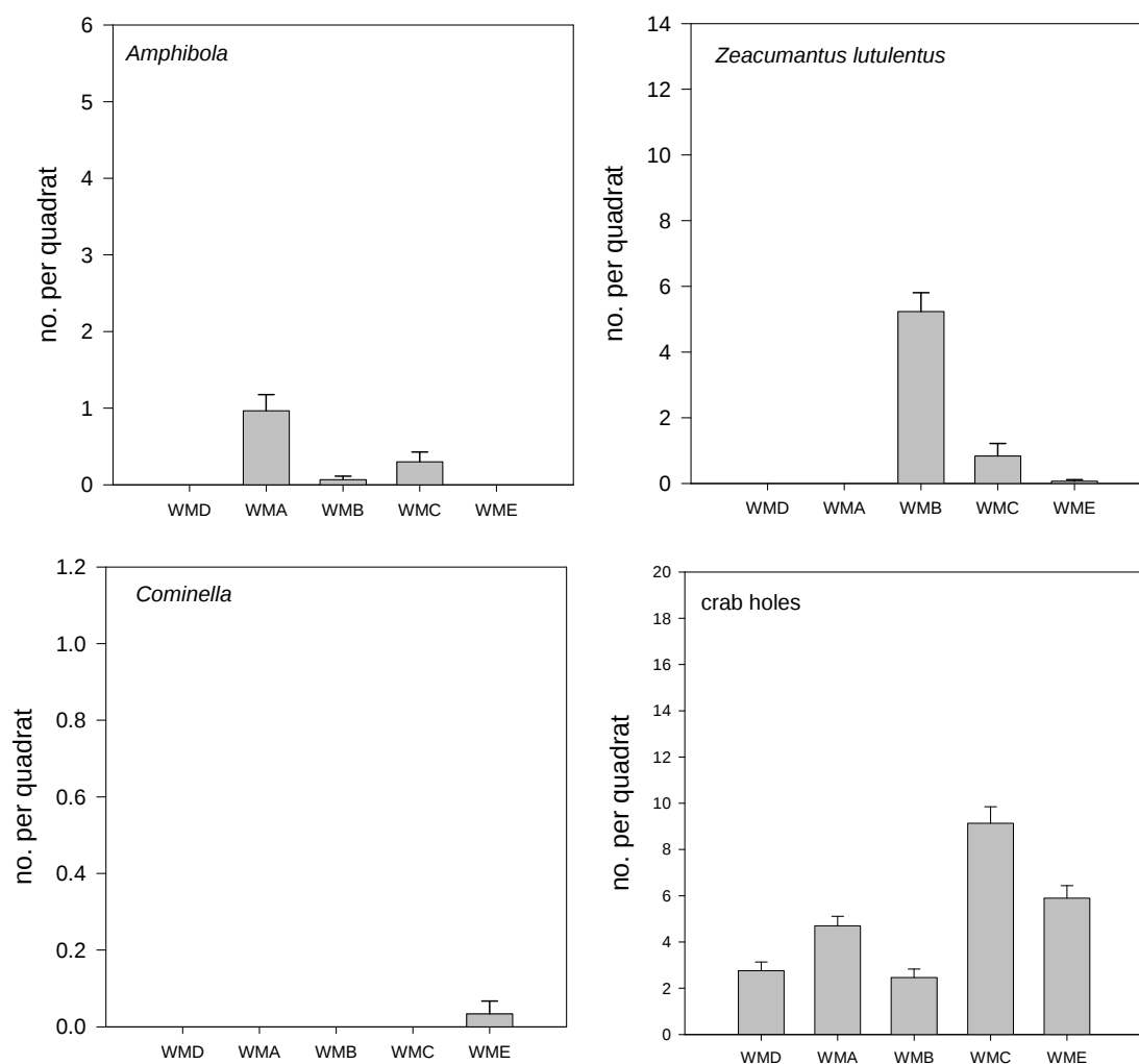
Figure 6: Abundance of surface macrofauna at sites WMD (intact mangrove habitat); WMA (cleared and mown 2005); WMB (cleared 2005); WMC (cleared 2007) and WME (bare intertidal flats).
