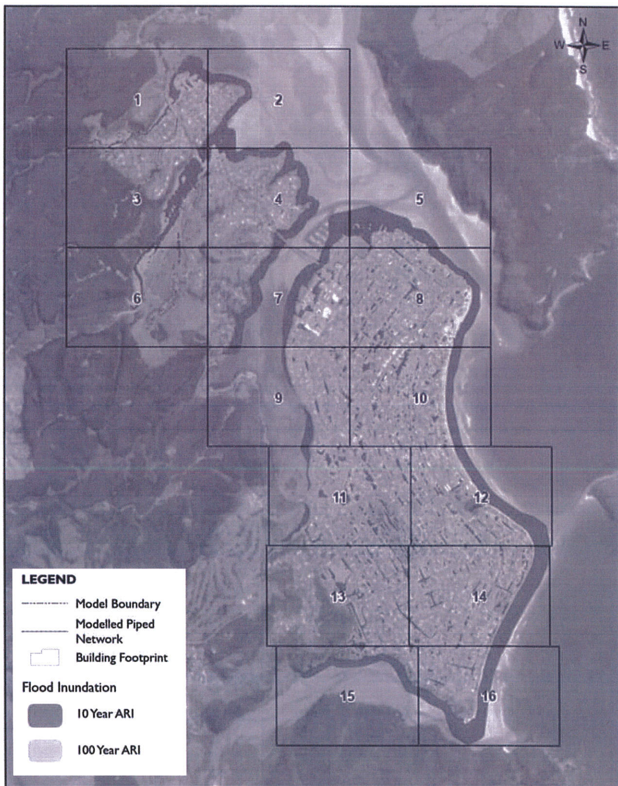
Figure 5-1: Flood Inundation Map Grid – 10 & 100 year ARI MPD 24 hour event
