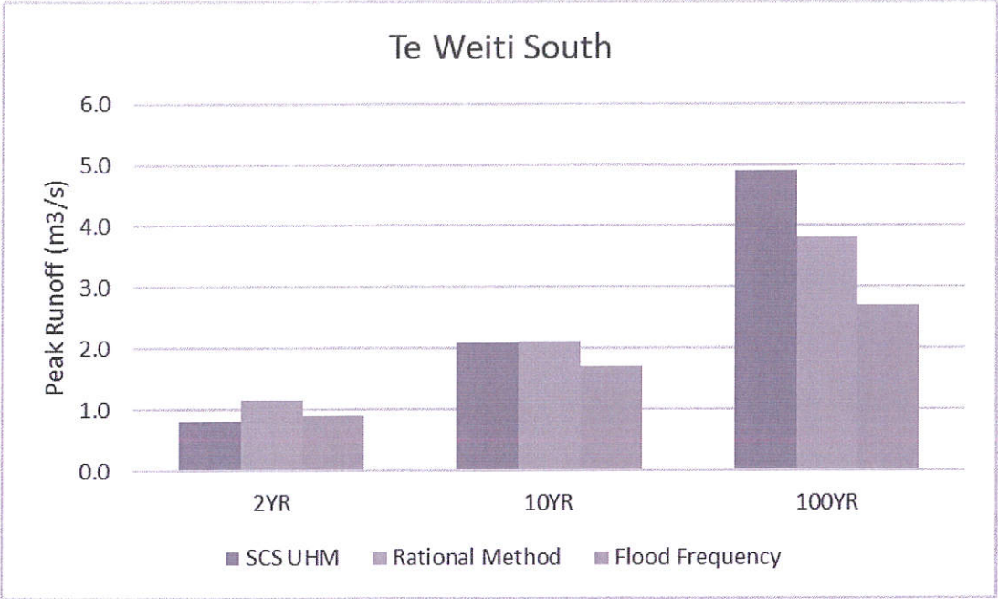
Figure 4-2 Te Weiti South Peak Flow Validation
