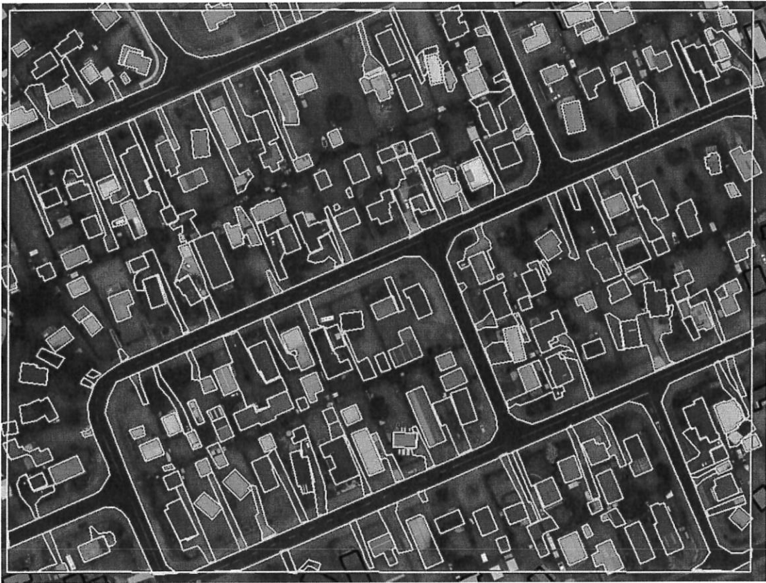
Figure 3-5 Sample area to calculate impervious footprint of other hard stand impervious areas
