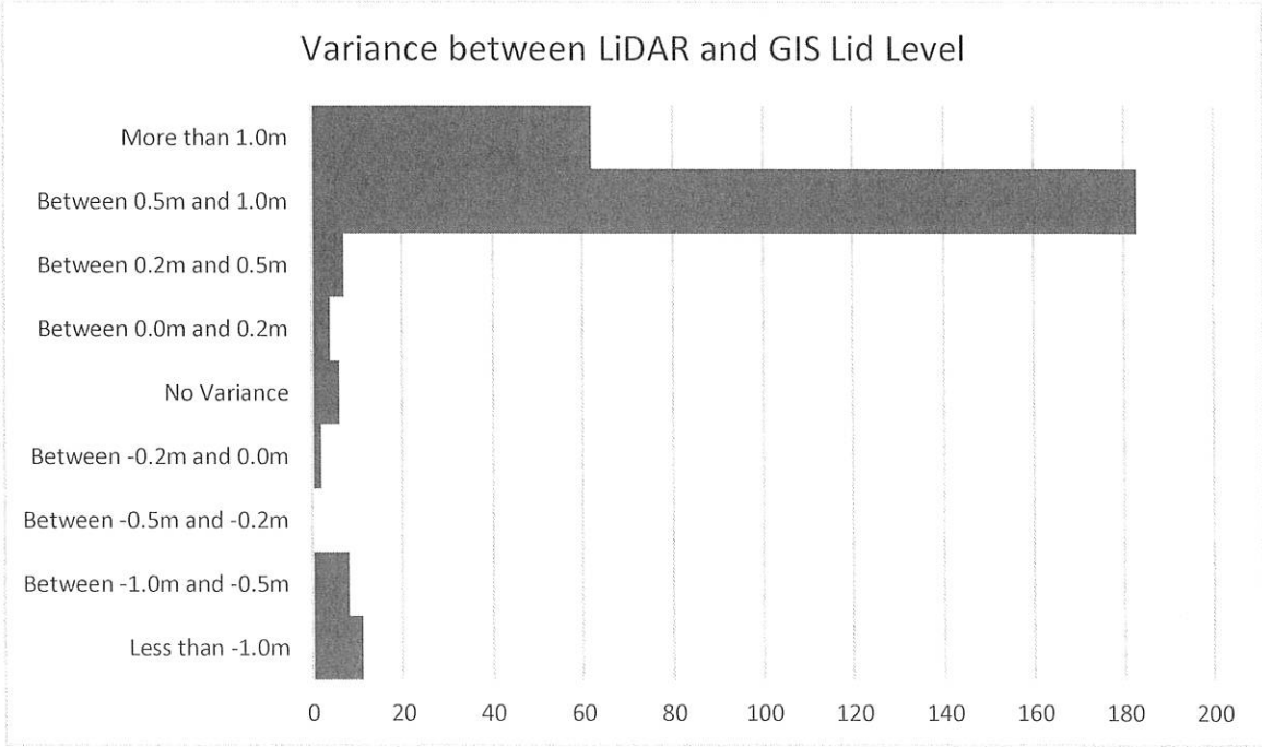
Figure 3-2 Variance between LiDAR and GIS Lid Level
