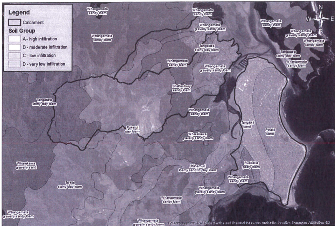
Figure 2-4 Model Domain Hydrological Soil Groups
