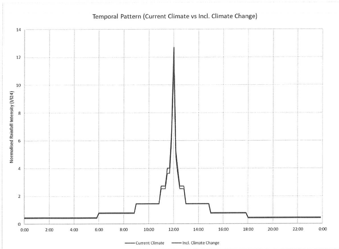
Figure 3-3 Temporal Pattern 24-hour Design Rainfall Event
