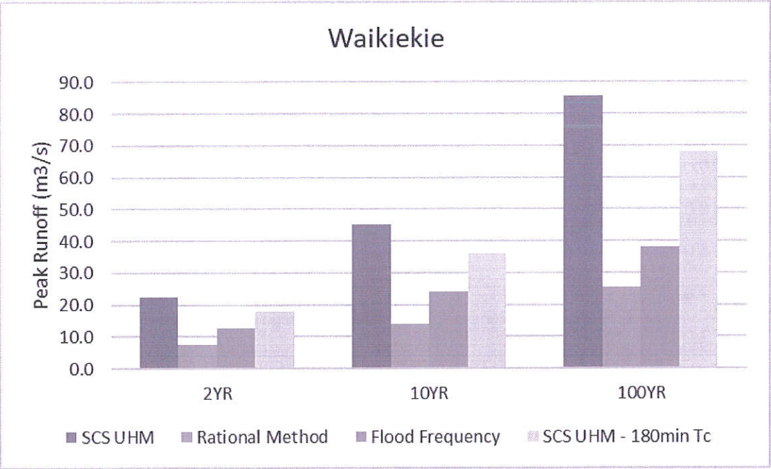
Figure 4-3 Waikiekie Peak Flow Validation 1
