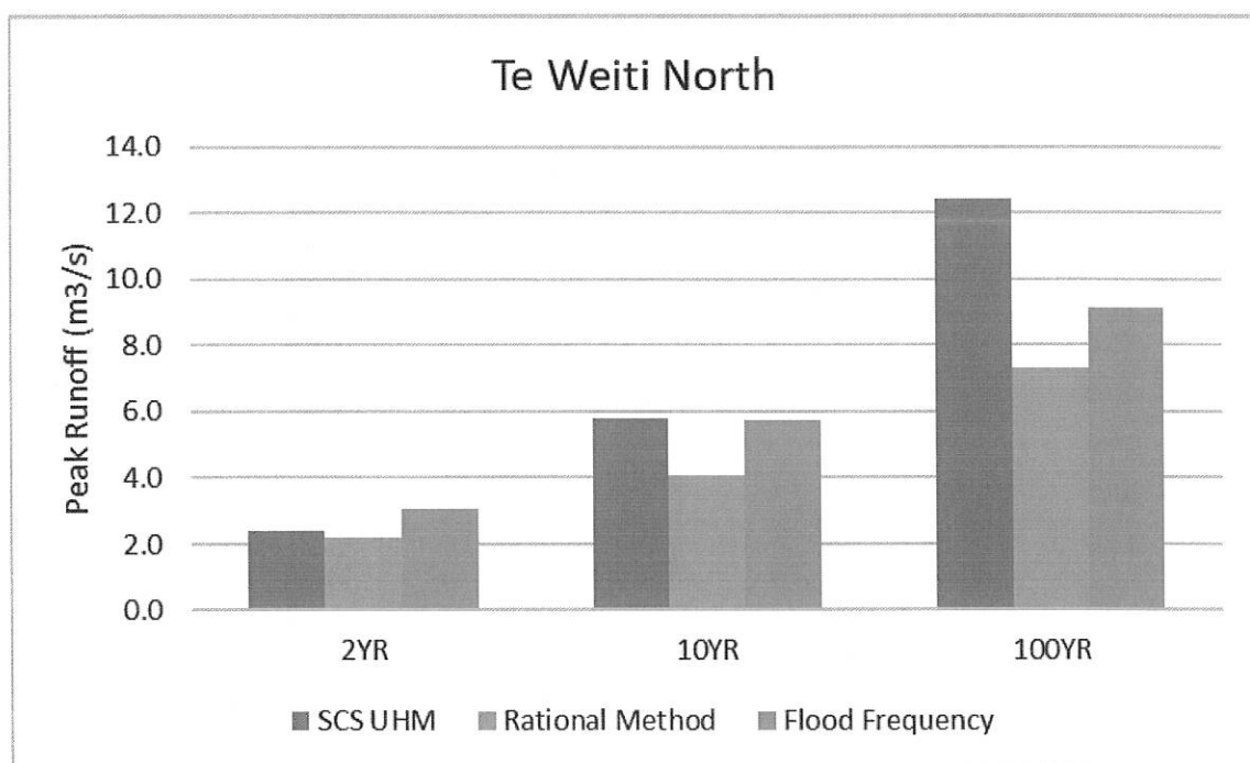
Figure 4-1 Te Weiti North Peak Flow Validation
