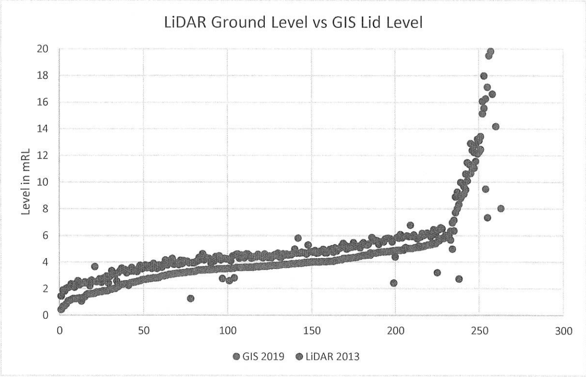
Figure 3-1 LiDAR Ground Level versus GIS Lid Level
