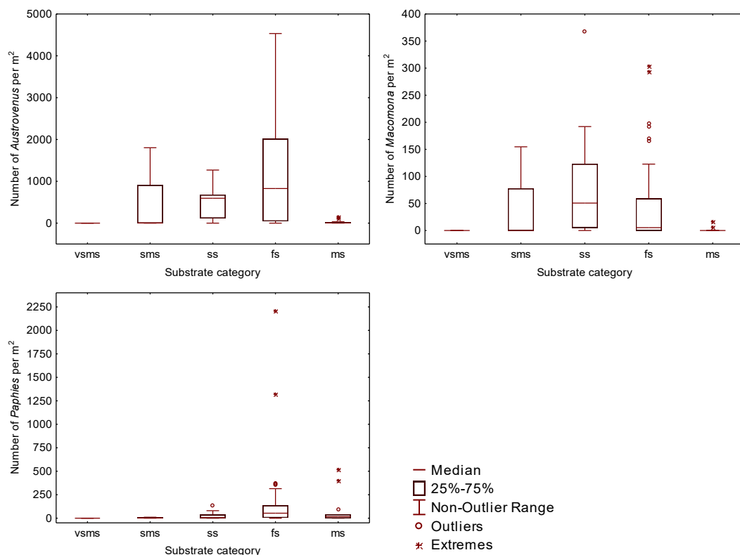
Figure 15: Boxplot showing the abundance of cockles ( Austrovenus stutchburyi ), wedge shells ( Macomona liliiana ) and pipi ( Paphies australis ) at sites classified into different substrate categories. Substrate categories: VSMS = Very soft mud / sand, SMS = Soft mud / sand, SS = Soft sand, FS = Firm sand; MS = Mobile sand.
