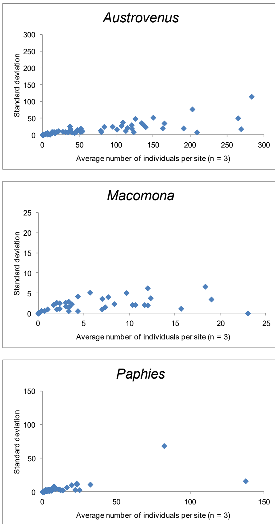
Figure D-1: Standard deviation of bivalve abundances calculated from three replicate samples.
